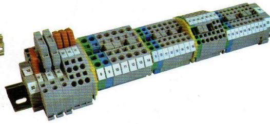
UJ Series Spring Cage Terminal Block
