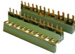
UP Series Comb Busbar
