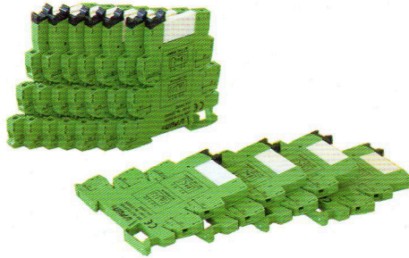
UDK Series Photoelectric / Relay-Coupling Terminal Block
